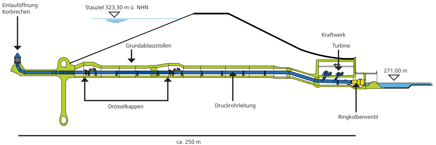
Turbine
